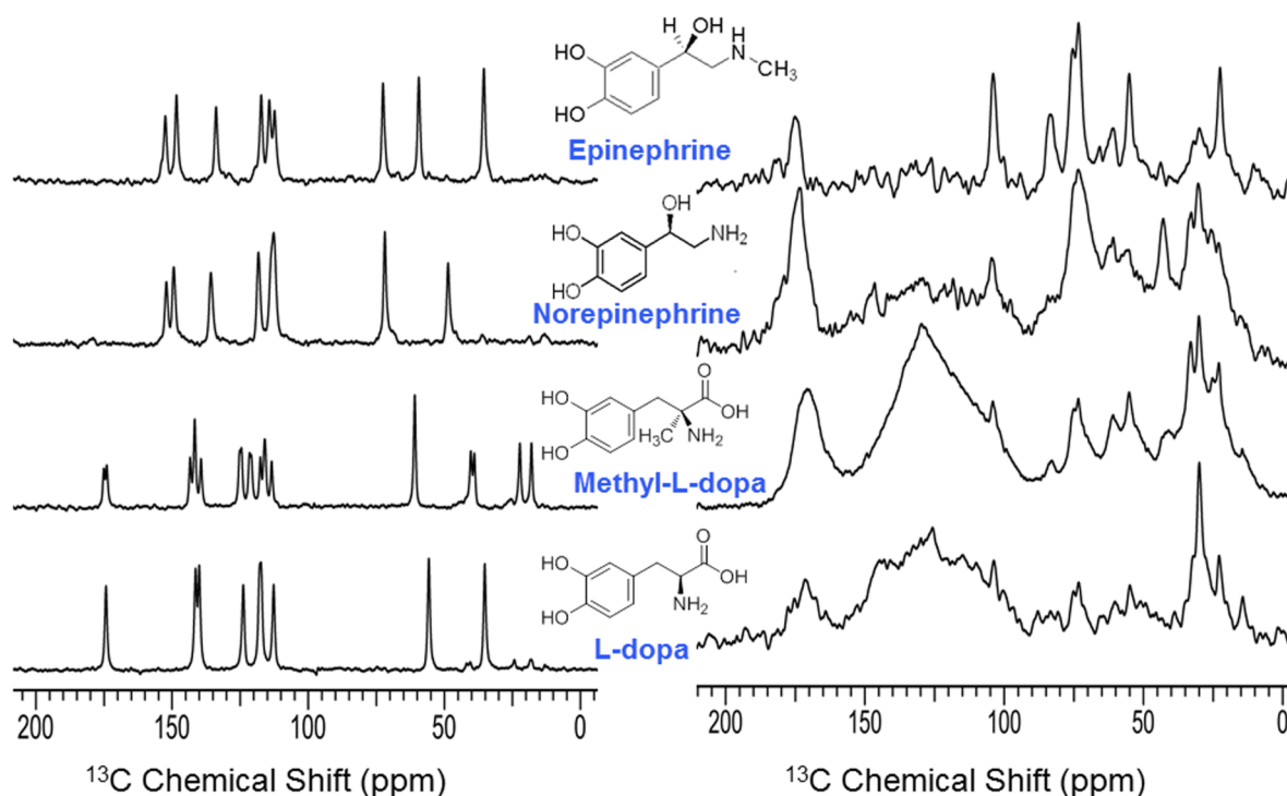
Figure 1. 150 MHz CPMAS solid-state ^{13}\text{C} spectra of catecholamine precursors and the resulting C. neoformans melanins obtained by in vitro biosynthesis. Chemical shift differences among phenol carbons in the precursors ( \sim 140\text{--}150 ppm) are attributed to variations in hydrogen-bonding networks and crystal packing in the solid state.
